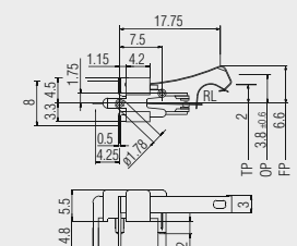
PCB terminal right angled 1010.9802
