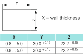
Basic types 1672, 1673 and 1675 single-pole illuminated / non-illuminated
