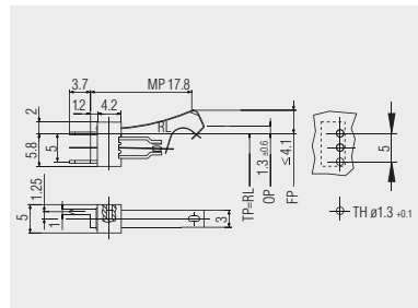
PCB terminal straight
