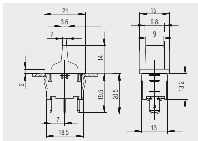
Quick-connect terminal 4.8 x 0.8 basic type 1818
